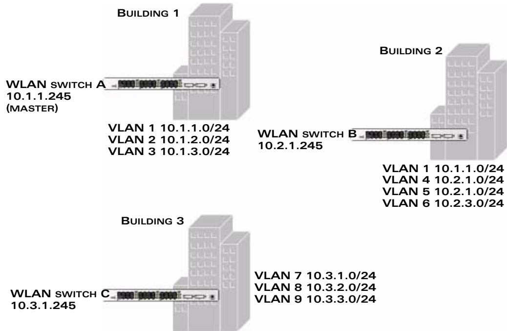
FIGURE 16-44 Example Configuration: Campus-Wide
