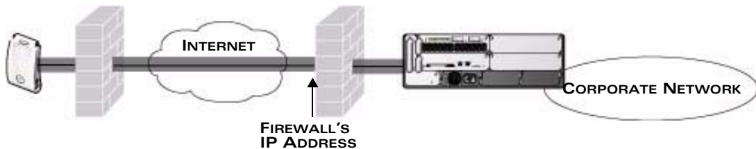
FIGURE 7-25 Remote AP with WLAN Switch Behind Firewall
