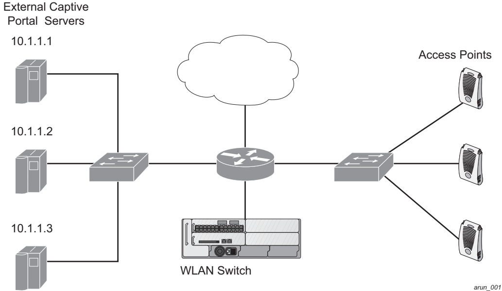
FIGURE 23-78 Example NAT-Mode Topology
