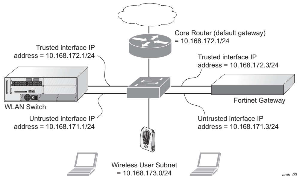
FIGURE 23-71 Example Route-Mode Topology
