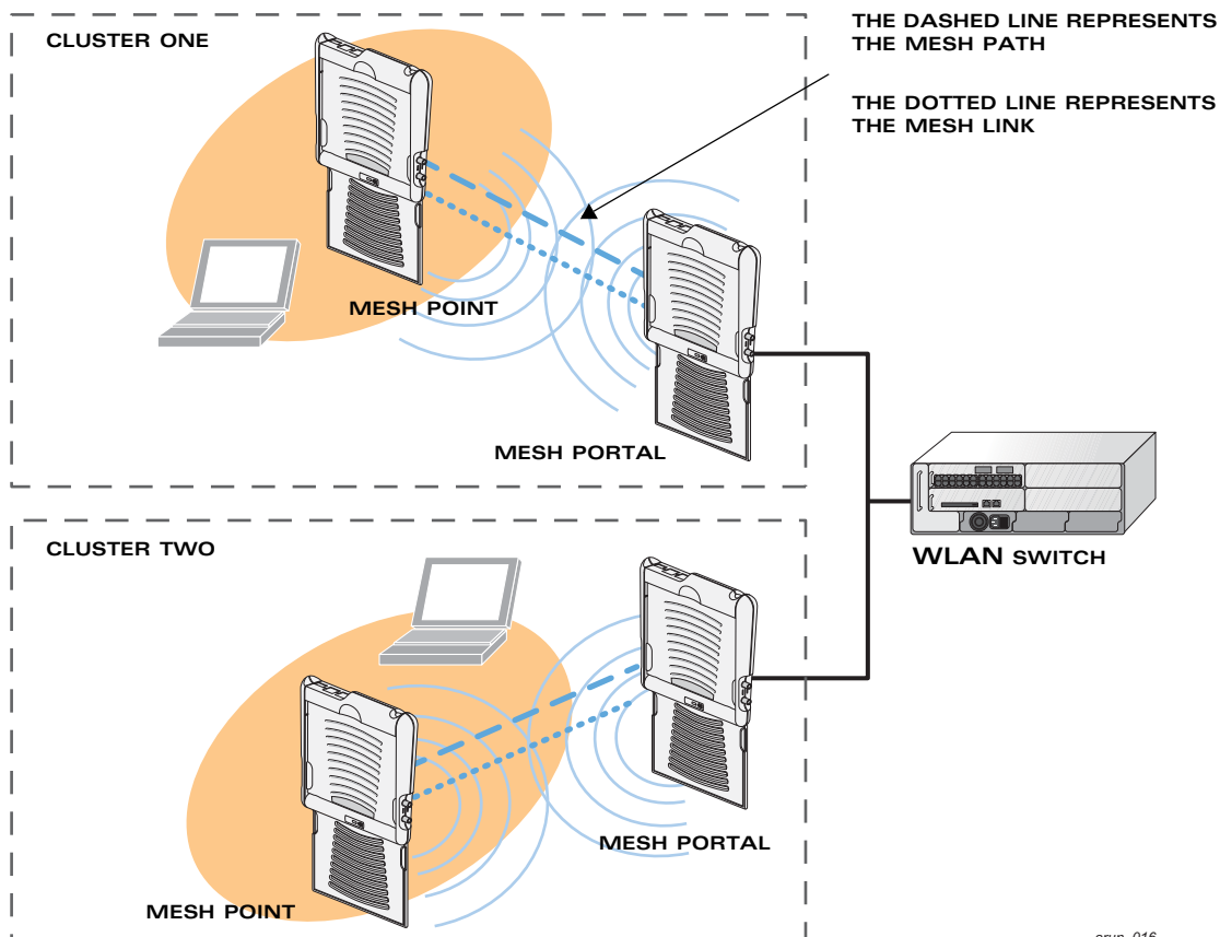
FIGURE 6-15 Sample Mesh Clusters
