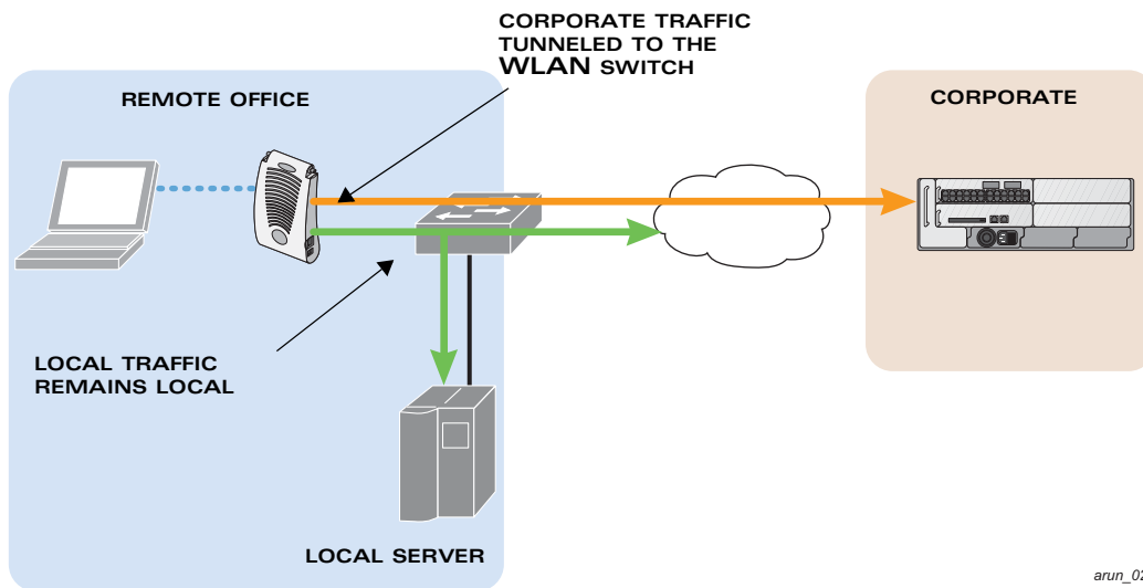
FIGURE 7-28 Sample Split Tunnel Environment
