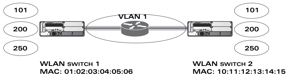
FIGURE 13-37 WLAN switch-to-WLAN switch xSec Example
