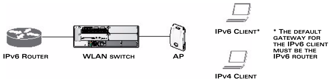
FIGURE 21-50 Supported Network Configuration
