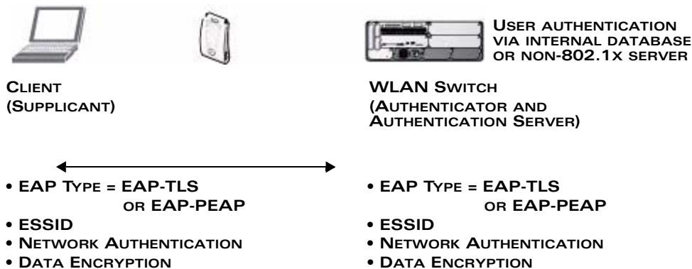
FIGURE 10-32 802.1x Authentication with Termination on WLAN Switch
