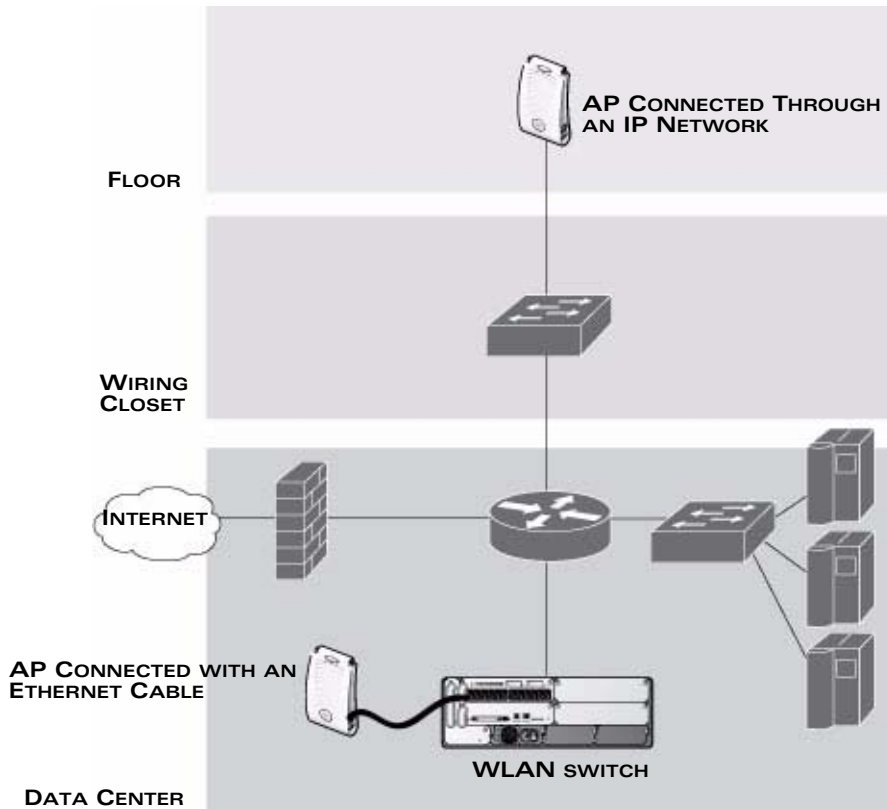
FIGURE 1-1 Connecting APs to the WLAN Switch
