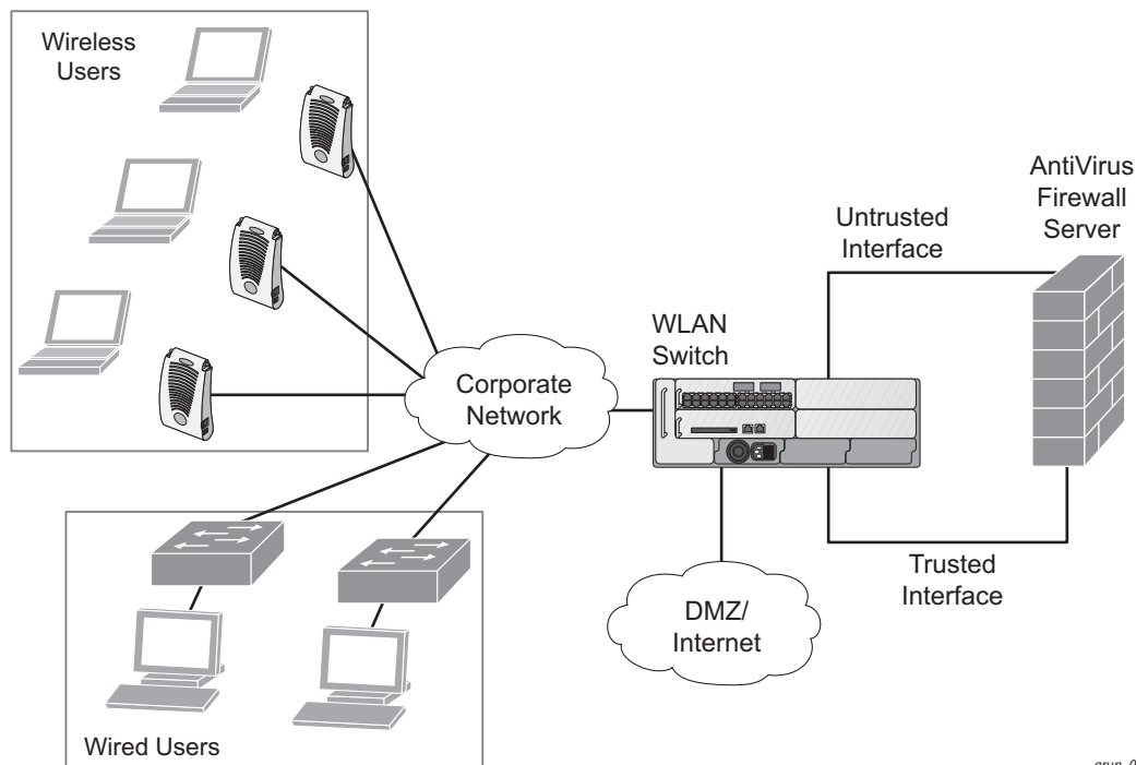
FIGURE 23-51 The ESI-Fortinet Topology
