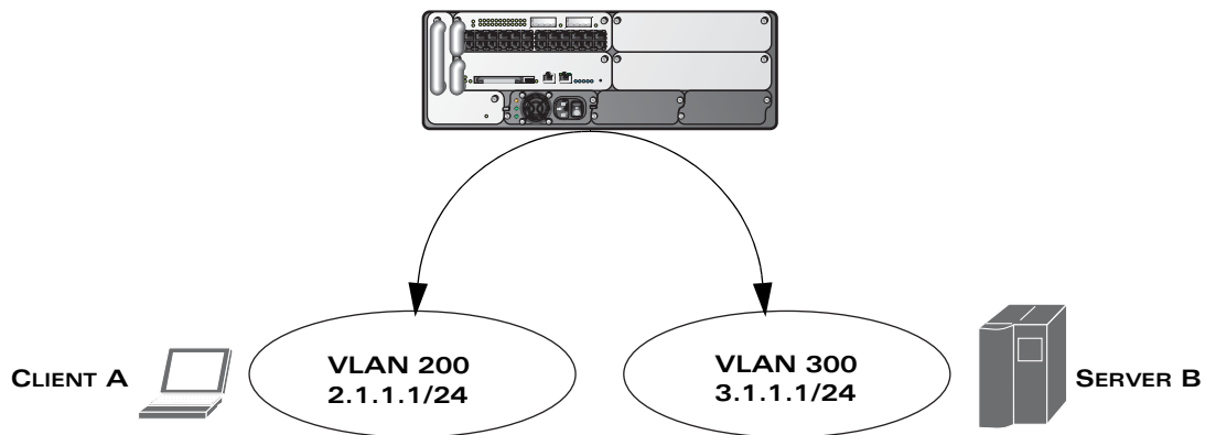
FIGURE 3-9 Default Inter-VLAN Routing
