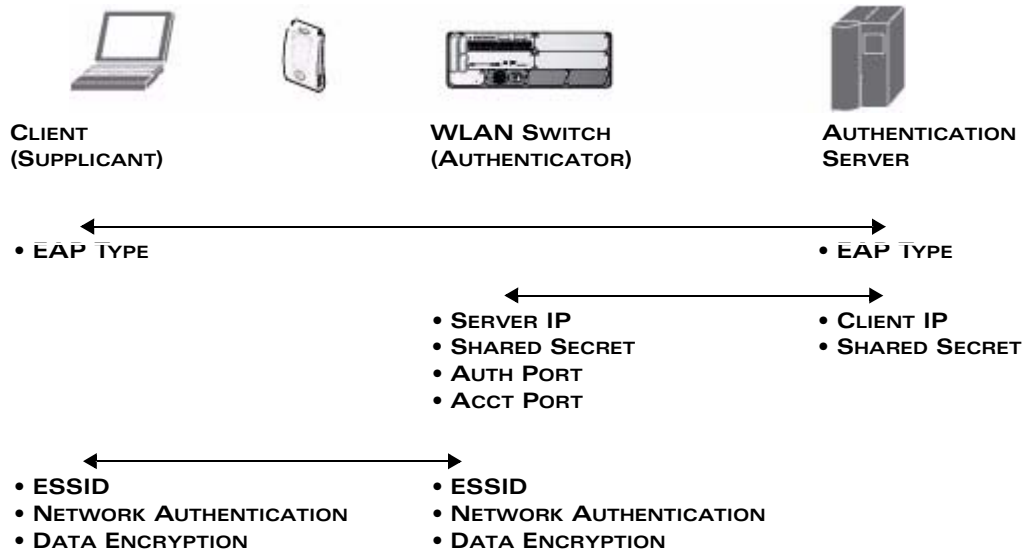
FIGURE 10-31 802.1x Authentication with RADIUS Server
