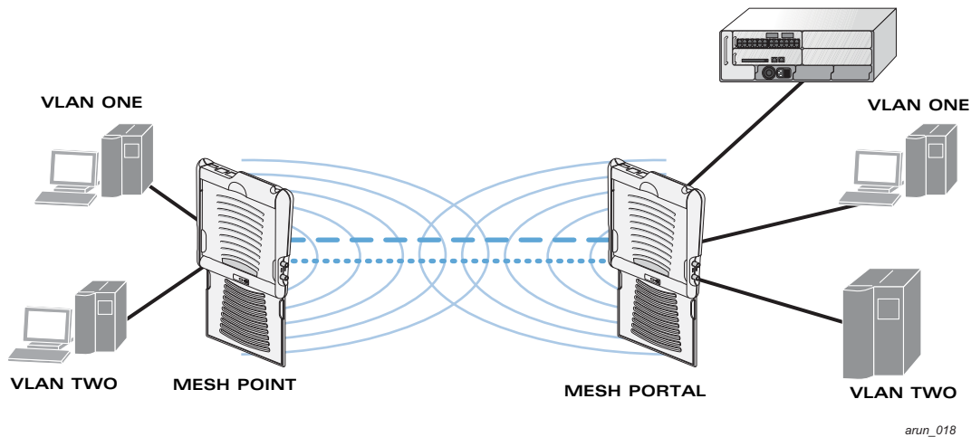
FIGURE 6-17 Sample Point-to-Point Deployment
