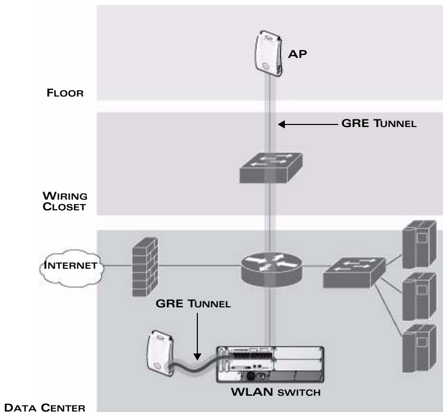
FIGURE 1-2 APs Establish GRE Tunnels to the WLAN Switch
