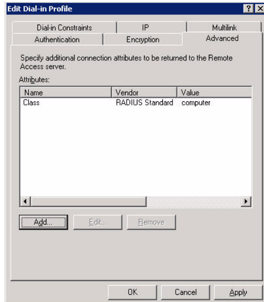
FIGURE D-94 Example RADIUS Class Attribute for “computer”
