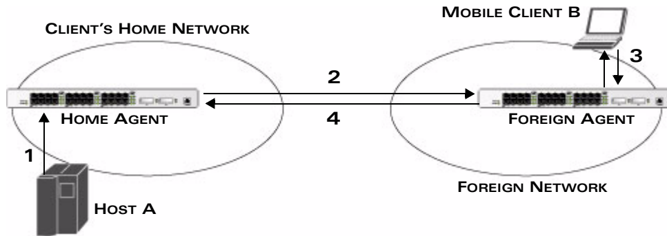
FIGURE 16-43 Routing of Traffic to Mobile Client within Mobility Domain
