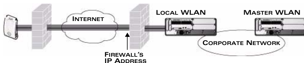
FIGURE 7-26 Remote AP in a Multi-WLAN Switch Environment
