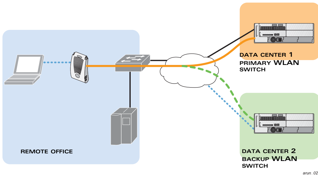
FIGURE 7-27 Sample Backup WLAN Switch Scenario
