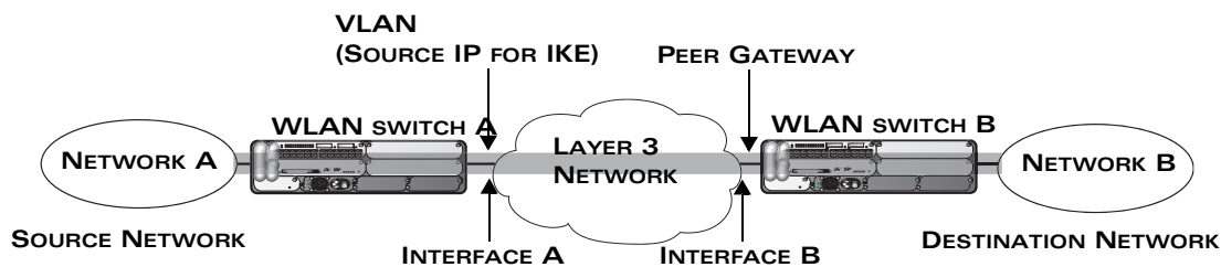
FIGURE 12-34 Site-to-Site VPN Configuration Components
