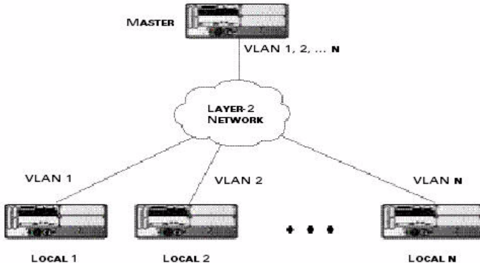
FIGURE 17-45 Redundant Topology: Master-Local Redundancy
