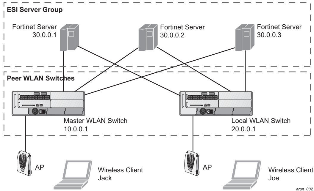
FIGURE 23-54 Peer WLAN Switches
